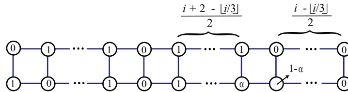
Figure 3: An illustration of labeling described in case 1a.
