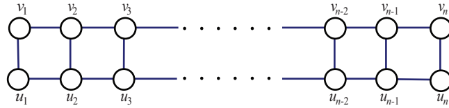
Figure 2: An illustration of P_2 \times P_n .
